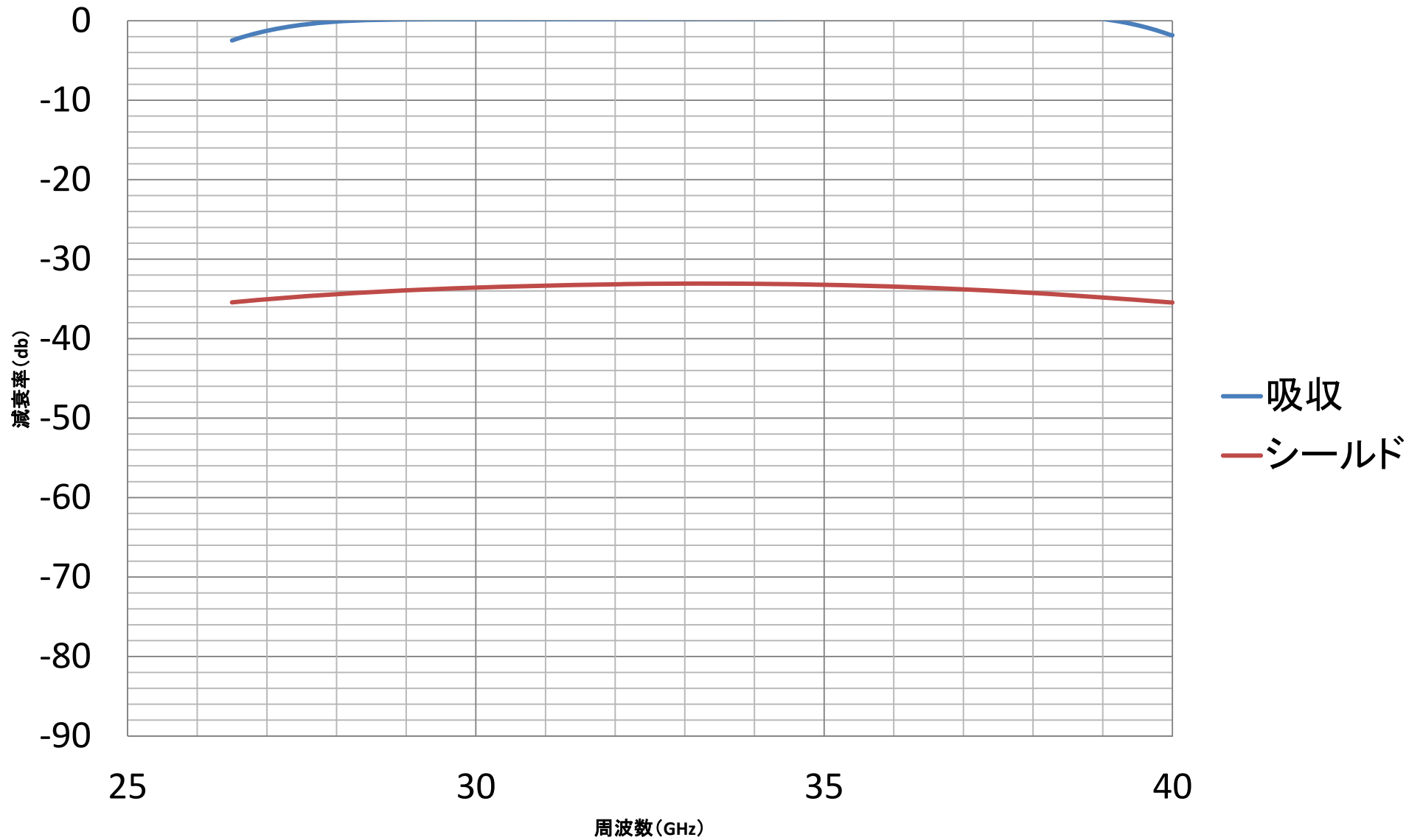
20150217[PCS-107AgCu (50 \mu m)] 26.5-40GHz
