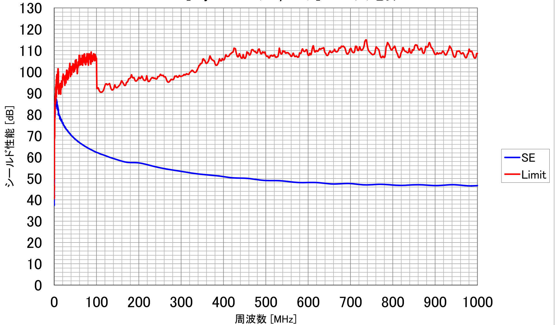
20150303[Plycalm-S(40 \mu m)]KEC 法電界
