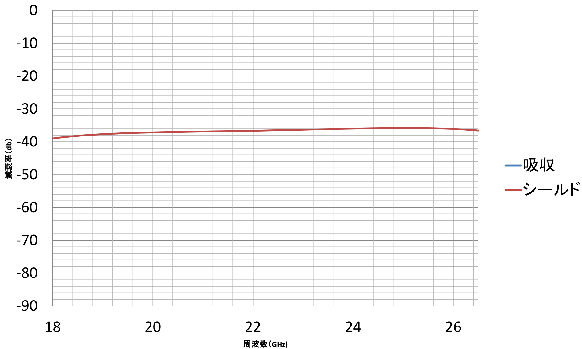
20150217[PCS-107AgCu(50 \mu m)] 18-26.5GHz
