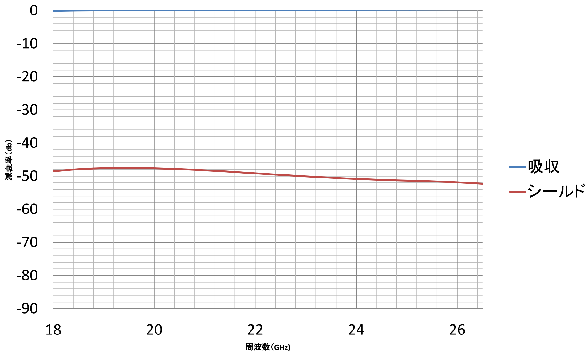
20150217[Polycalm-G 1501(35 \mu m)] 18-26.5GHz
