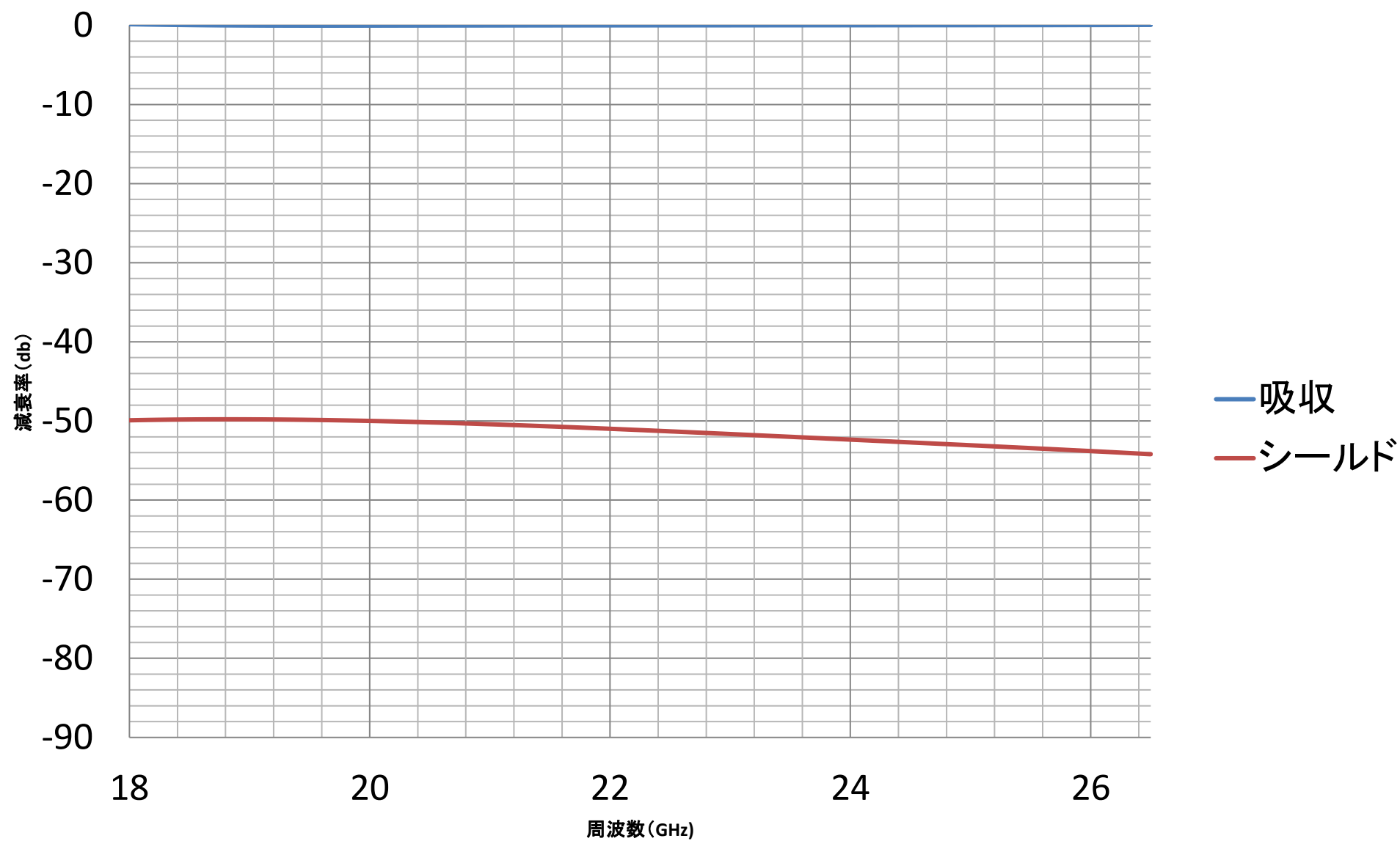
20210908-08_FS_18-26.5GHz_PCS-G2028_50μ
