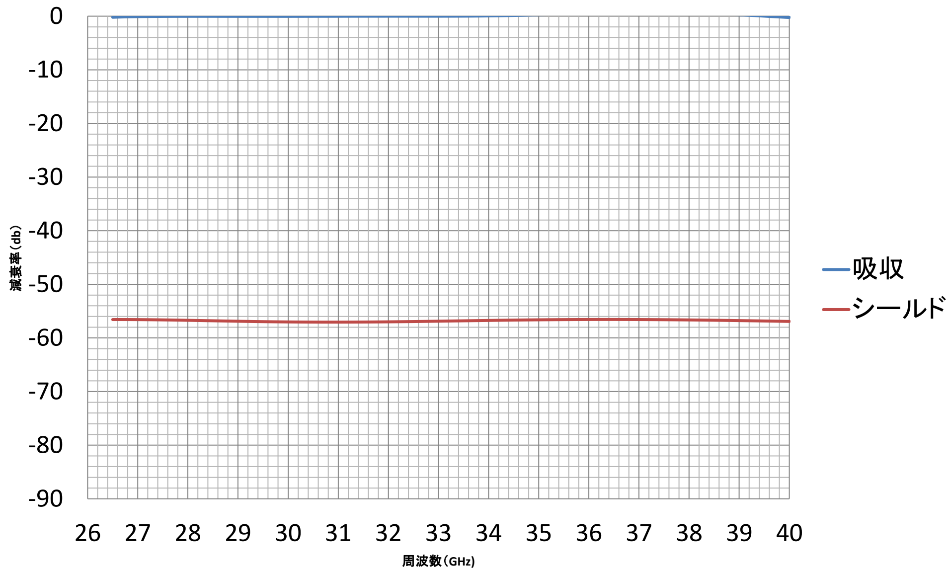
20210908-08_FS_26.5-40GHz_PCS-G2028_50μ
