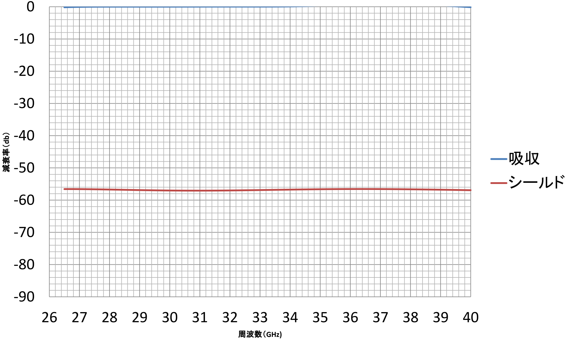
20210908-07_FS_26.5-40GHz_PCS-1950Ag_15μ
