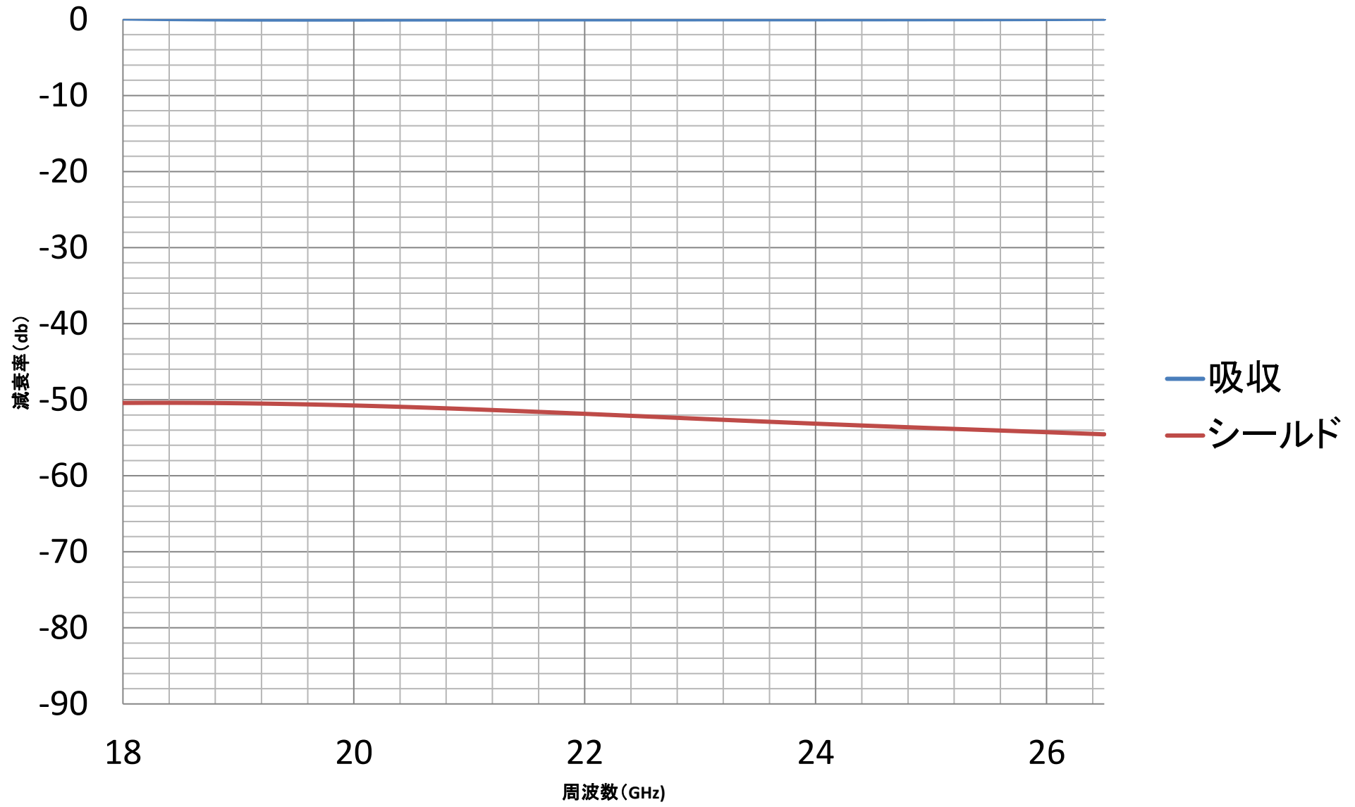
20210908-07_FS_18-26.5GHz_PCS-1950Ag_15μ
