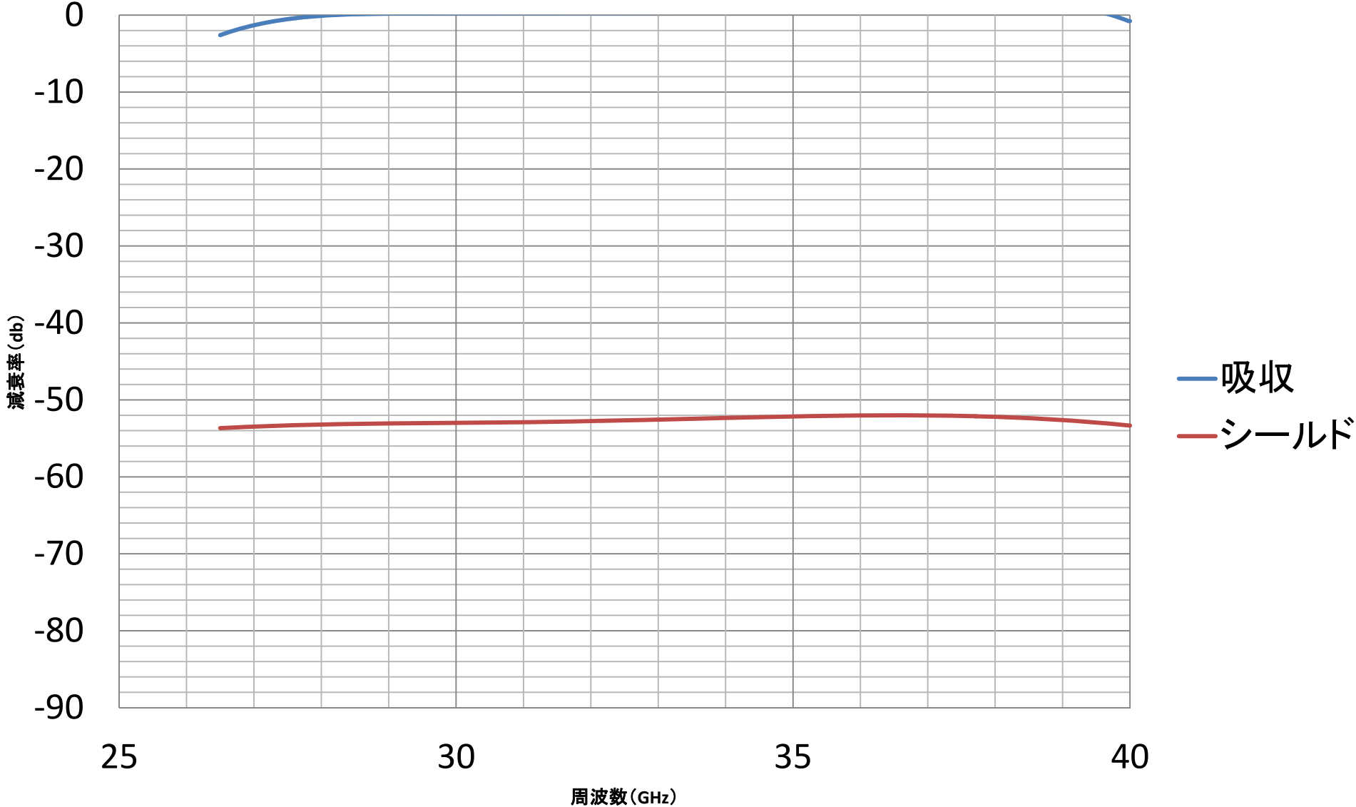
20150217[Polycalm-G 1501 (35 \mu m)] 26.5-40GHz
